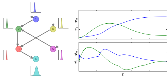
Fig. 3. (Left:) Graphical representation of the transition matrix and duration probabilities for each state. Note the three paths formed according to our 3 demonstrations in (Fig. 2(a)). (Right:) Executed motion on the remote side, using the learned TP-HSMM and the MPC controller.
