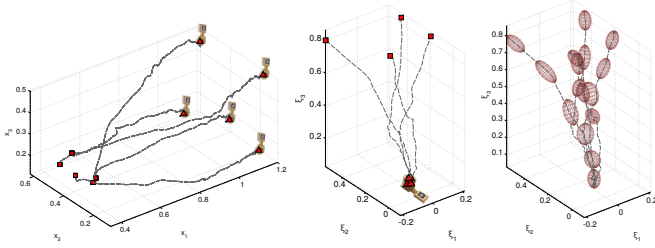
Fig. 6. Left : Demonstrations of the motion in the global frame. Middle : The motions projected to the task-parametrized frame of the receptacle. Right : The TP-HSMM model learned online from the demonstrations in the task-parametrized frame of the receptacle.
