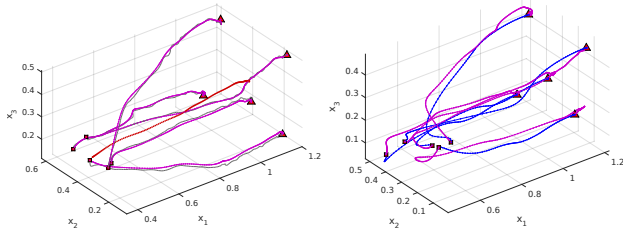
Fig. 8. Left : Demonstrations (in grey) used to learn the ProMP model along with reproductions (in purple) using ProMP on the start and target points taken from the demonstrations. The red dotted line represents the mean of the trajectory distribution. Right : Motions generated with our system (in blue) and with the ProMP method (in purple), based on the same start and target points.
