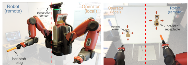
Fig. 5. Experimental setup of teleoperation mock-up with the Baxter robot. The operator uses the left arm to provide demonstrations and directly teleoperate the remote (right) arm. Once the TP-HSMM model is learned, the remote side (robot) can autonomously execute the hot-stabbing motion, successfully adapting to changing receptacle locations.
