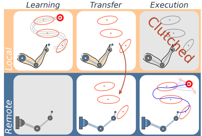
Fig. 1. Overview of supervisory teleoperation within our approach. Top : Local system where a teleoperator is using an exoskeleton to demonstrate motions to the system and to perform direct teleoperation whenever necessary. Bottom : Remote side where a robotic manipulator receives a learned model of the task at hand and can then execute the task autonomously using local feedback. During autonomous execution, the overall system is clutched, i.e. the state of the local system does not affect the state evolution on the remote side.
